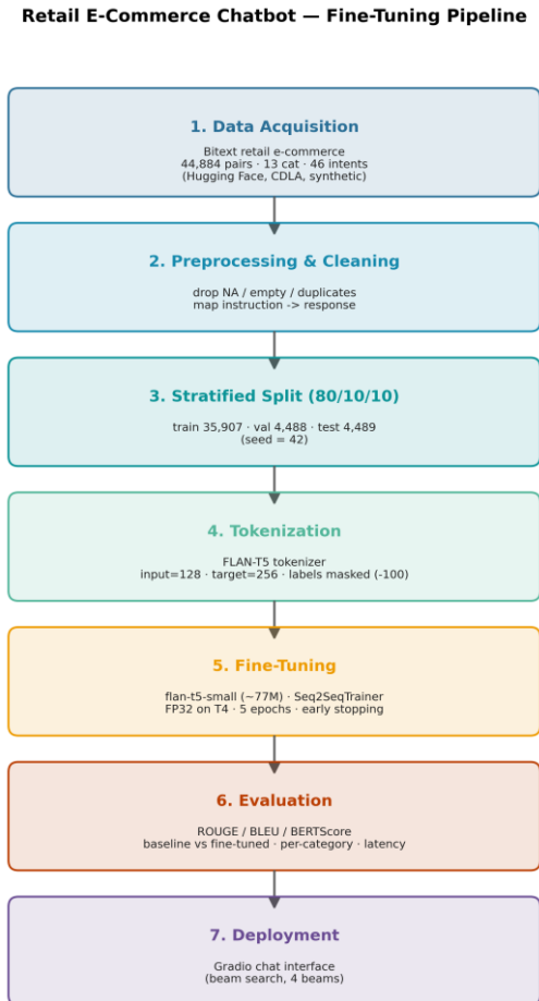
Fig. 8. End-to-end fine-tuning pipeline (data acquisition \rightarrow preprocessing \rightarrow stratified split \rightarrow tokenization \rightarrow fine-tuning \rightarrow evaluation \rightarrow deployment).
