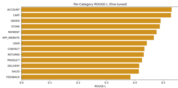
Fig. 6. Per-category ROUGE-L of the fine-tuned model.
